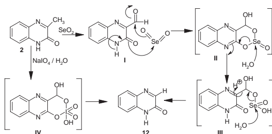
Scheme 1. Plausible mechanism for the formation of 12 from 2 by \text{SeO}_2 or \text{NaIO}_4 .
